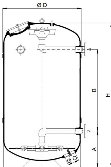
Top diffuser
