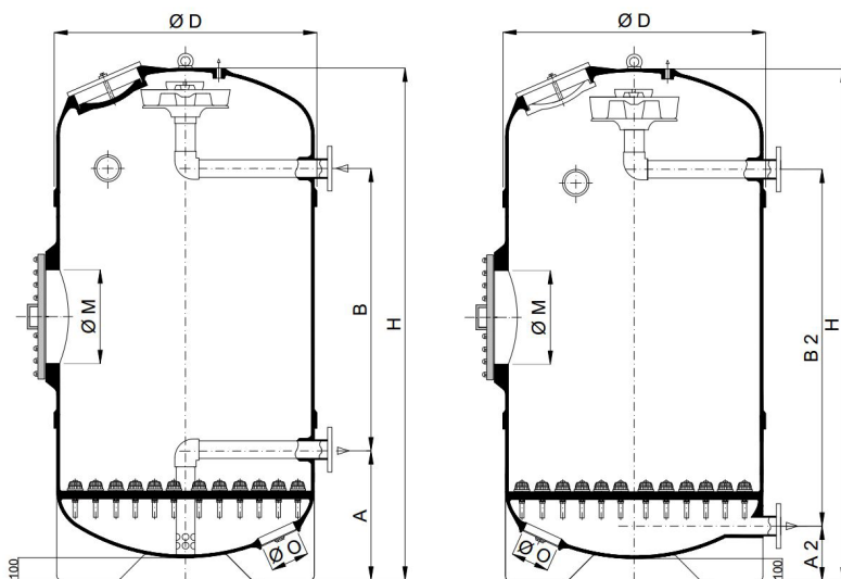
Flange integrated in body
